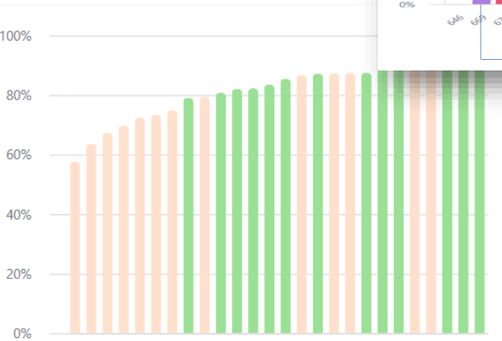
TRUST SCORES
