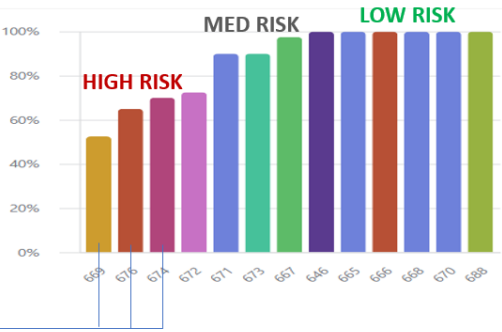
STRESS SCORES
